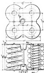
Figs. 4534-4535. Four-Coil Truck Bolster Spring.
